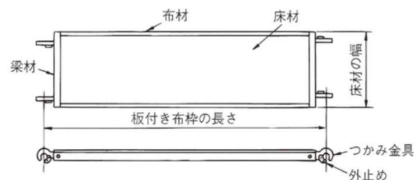
板付き布枠
